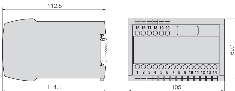
Fig. 6. SINEAX M 563 in housing P20/105 clipped onto a top-hat rail (35 × 15 mm or 35 × 7.5 mm, acc. to EN 50 022).
